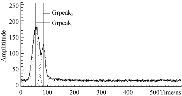
Fig 10 Simulated waveform Dotted curve shows two Gaussian distribution decomposed from the same data set shown in Fig 9
