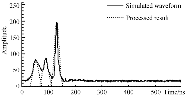
Fig 8 A simulated waveform and processed result by the proposed algorithm
