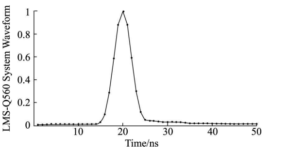
Fig. 2 System waveform of REGL LMS-Q560
