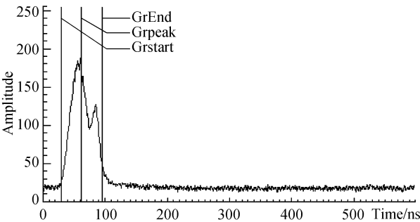
Fig 9 Ground location of SLICER
