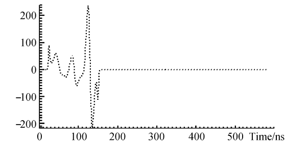
Fig 6 First derivative of waveform
