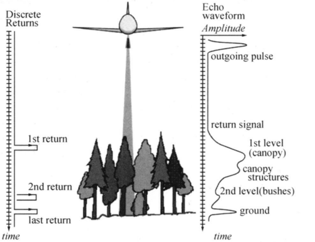
Fig. 1 Full waveform data and discrete echo (Optech, 2006)
