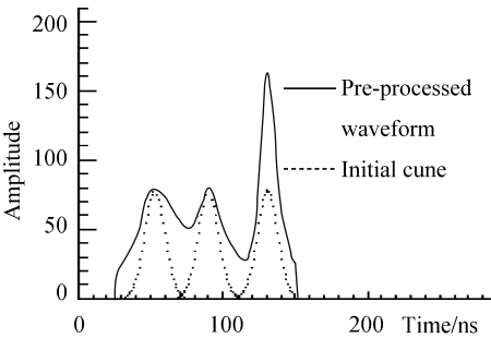
Fig 7 Waveform with initial values estimated
