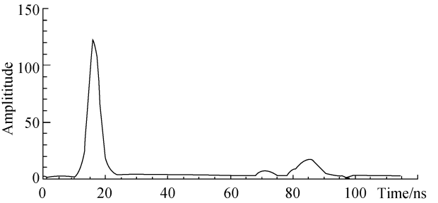
Fig 13 Raw waveform data acquired by RIEGL IM5600
